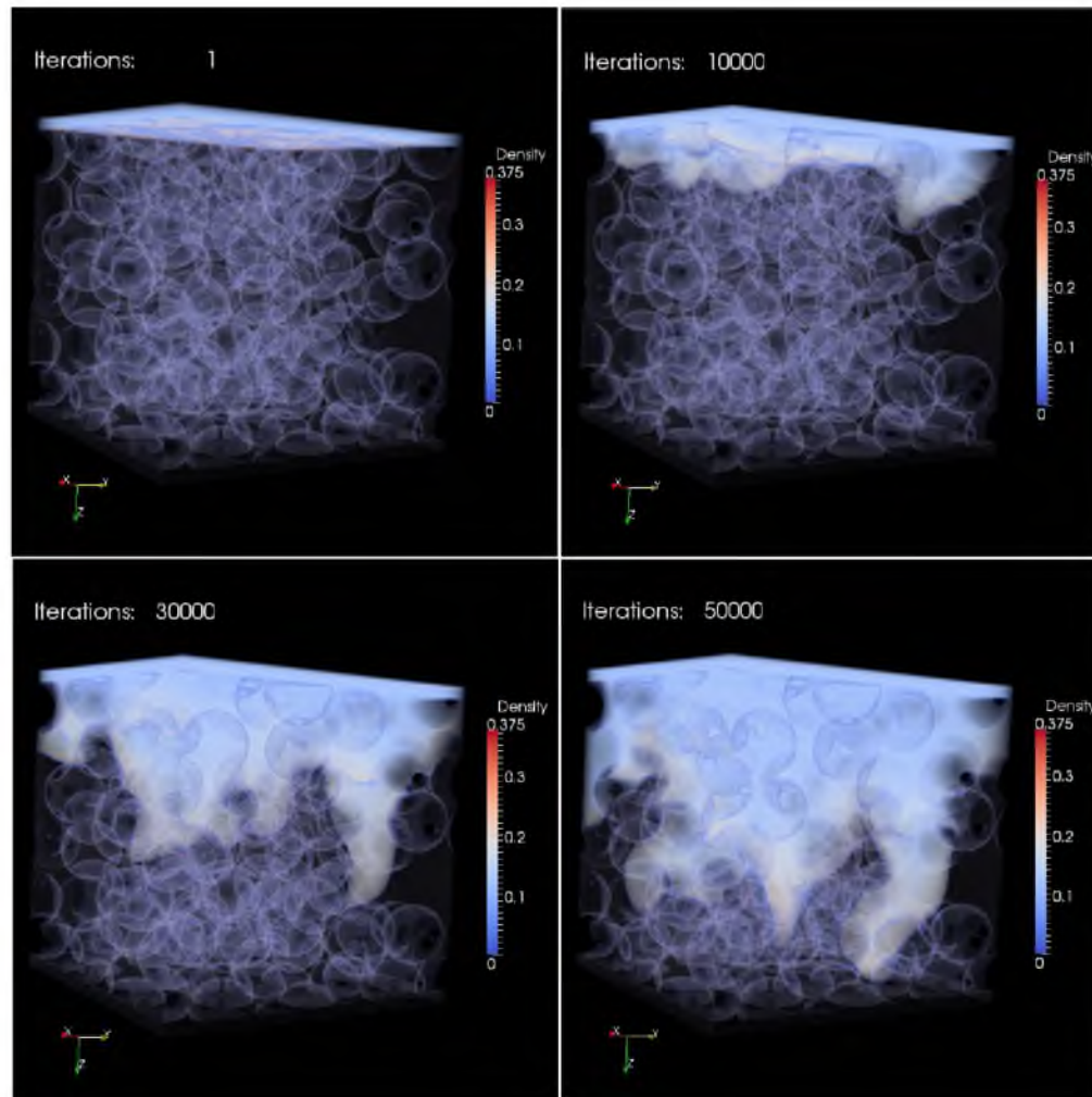
Figure 5.6: Sequence of simulations of two-phase flow in a packed bed of hydrophilic glass beads particles ( 200 \times 240 \mu\text{m} ). Percolation simulations by the single component He-Chan-Zhang LBM. (Density ratio = 1/3 ; Lattice size of 256 \times 256 \times 256 voxels; Images for 1, 10,000, 30,000 and 50,000 iterations).
