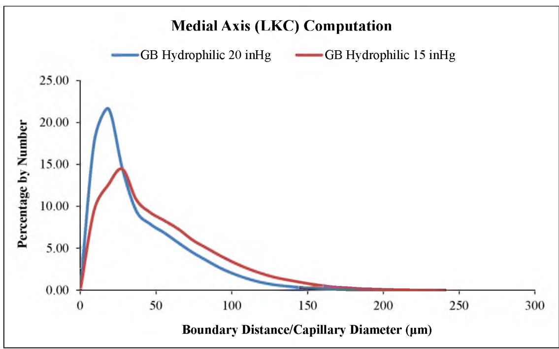
Figure 4.2: Medial axis pore analysis of the hydrophilic glass beads (200 x 240 µm) filter cakes tested at initial vacuum pressure of 20 inHg and 15 inHg, respectively.
