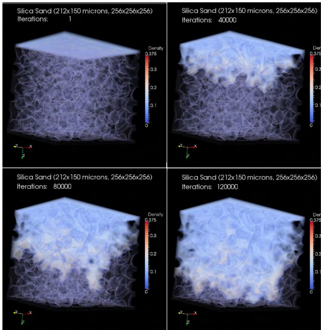
Figure 5.7: Sequence of simulations of two-phase flow in a packed bed of silica sand particles (particle size 150 x 212 \mu\text{m} ). Percolation simulations by the single component He-Chan-Zhang LBM. (Density ratio = 1/3; Lattice size of 256 x 256 x 256 voxels; Images in increments of 40,000 iteration steps each).
