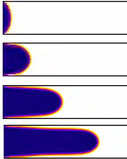
Figure 1.4: Simulations of fluid displacement for increasing difference in pressure controlled by the density at the outlet, which has values from top to bottom: 0.2508, 0.2498, 0.2482, and 0.2466. D2Q9 lattice of size 35 \times 130 \text{ lu}^2 . Parameters for simulations are \bar{k} = 0.1 , D_\rho = 0.99 , and \rho_l/\rho_g = 10 .
