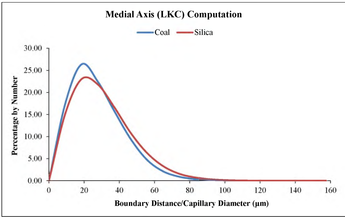
Figure 4.1: Medial axis pore analysis of the coal and silica (149 x 250 µm) filter cakes.
