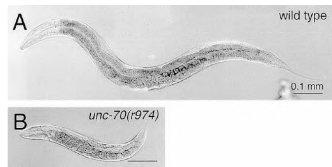
Figure 1. Light microscope images of (A) wild-type and (B) unc-70(r974) adult animals.
