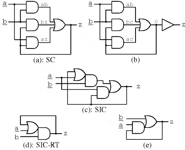
Figure 3. Static C-Elements: (a) C-Element with hazards, (b) locally timed, (c) Speed-Independent, (d) with RT assumption \underline{a}\downarrow < \underline{b}\downarrow , (e) with RT assumption \underline{a}\uparrow < \underline{b}\uparrow
