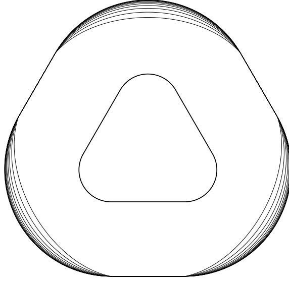
Figure 3.5. Error function convergence to zero, for three 120 degrees arcs in curve. in C(t) so close that the offset curve in those regions intersects itself. This type of loop is referred to as a global loop .
