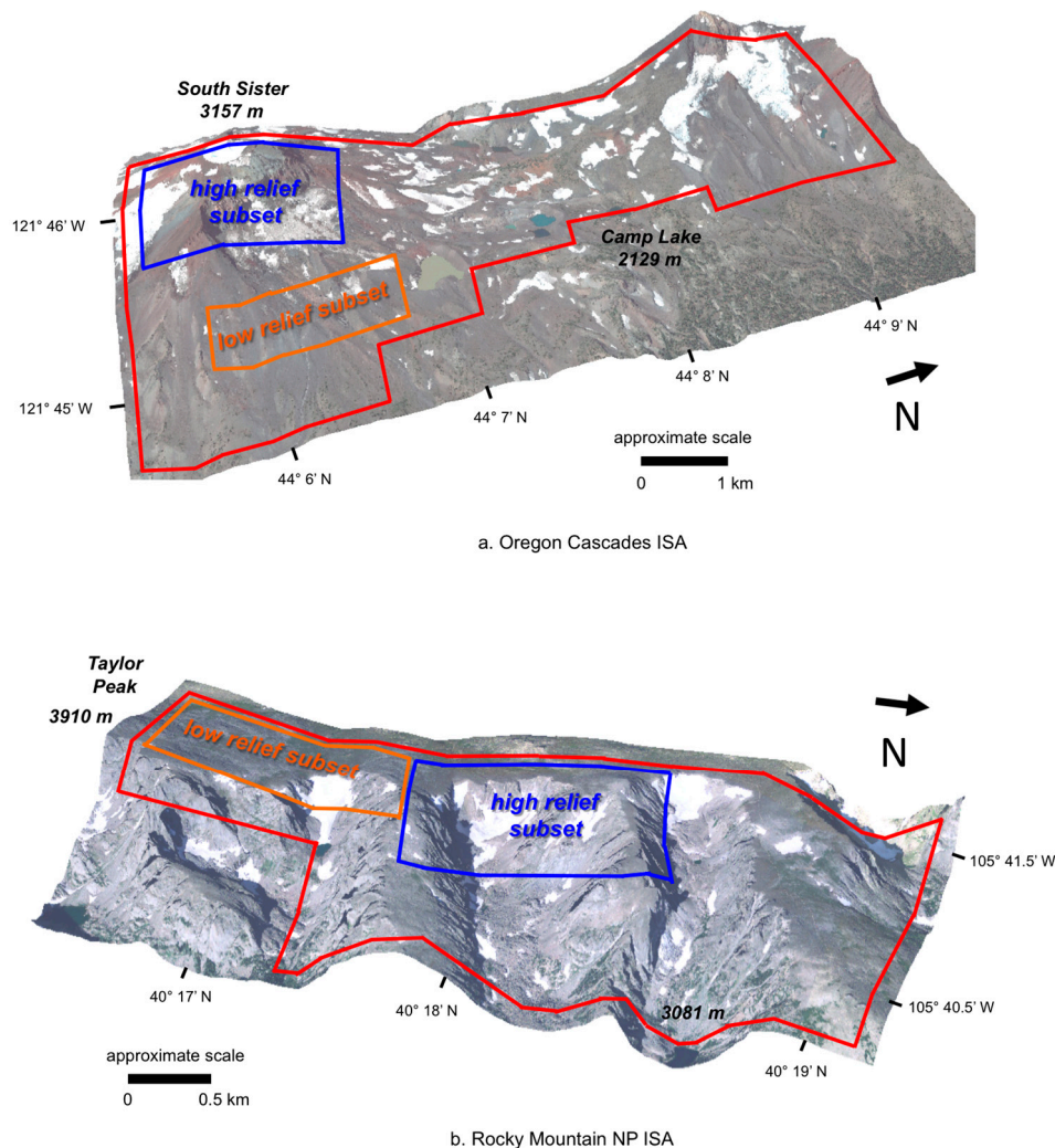
Figure 2. (a) Oregon Cascades ISA and (b) Rocky Mountain NP ISA. Extent of ISA is outlined in red, while the extent of high-relief subsets are outlined in blue and low-relief subsets are outlined in orange. Image sources: Digital elevation models for both study areas are from the National Elevation Dataset (NED) [50]. Draped imagery for the Oregon Cascades ISA is from 0.4 m pan-sharpened natural color WorldView 2 imagery, acquired 1 September 2013. Draped imagery for the Rocky Mountain NP ISA is from 1 m aerial orthoimagery available from the National Map [51], precise acquisition date not available.
