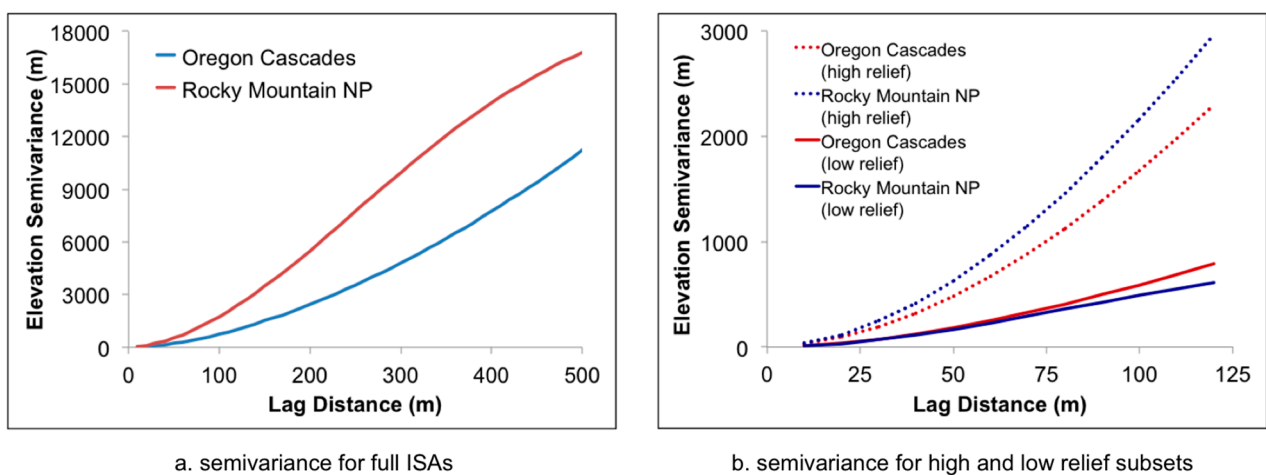
Figure 3. Semivariograms for elevation derived from 10 m DEM for (a) the Oregon Cascades and Rocky Mountain NP ISAs, and (b) high- and low-relief subsets from the Oregon Cascades and Rocky Mountain NP ISAs.
