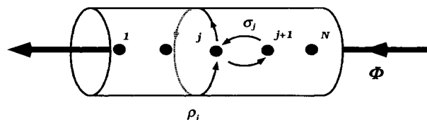
FIG. 1. Braid-group generators on a cylinder. \Phi is the central flux through the hole.
