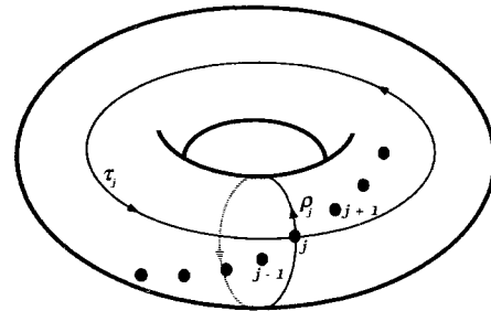
FIG. 2. Braid-group generators \rho_j and \tau_j on a torus.
