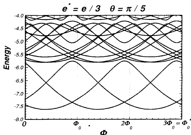
FIG. 3. Spectral flow of a three-anyon system on a 3 \times 3 cylindrical lattice. The statistics is \pi/5 and the charge is e/3 .
