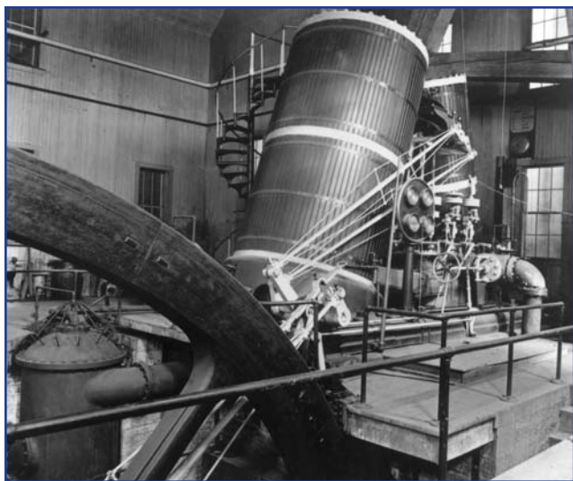
Cornish pump at the Ontario mine. Photo courtesy of the Utah State Historical Society.
