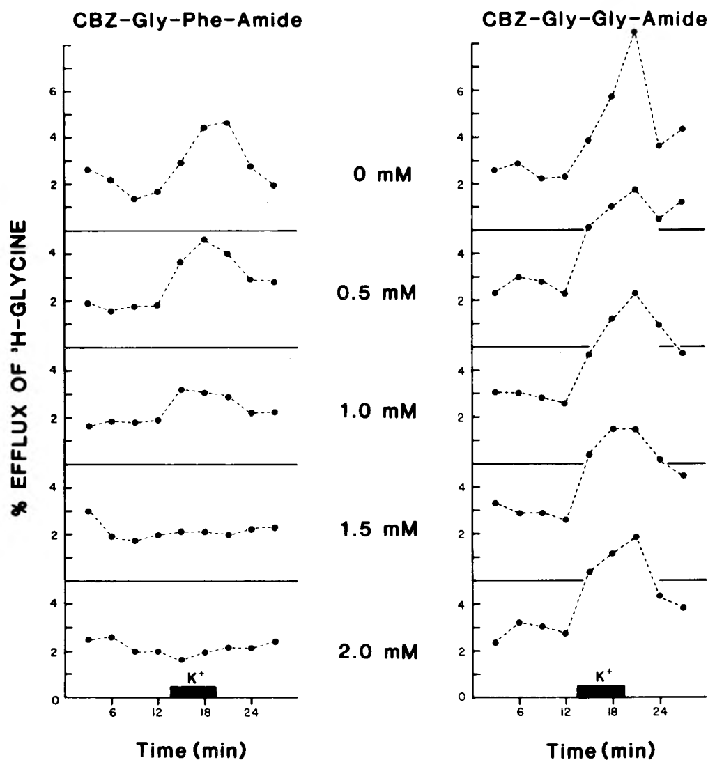
Figure 7. Specificity and dose-dependent inhibition by CBZ-dipeptide amides of K^+ -stimulated [ ^3H ]glycine release. Retinas preloaded with [ ^3H ]glycine were incubated with either CBZ-Gly-Phe-amide (left) or CBZ-Gly-Gly-amide (right). The K^+ -stimulated efflux of [ ^3H ]glycine was reduced with increasing concentrations of CBZ-Gly-Phe-amide and was unaltered at any concentration of CBZ-Gly-Gly-amide.
