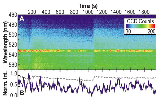
FIG. 3. (Color online) Temporal fluctuations of SHG from a single hot spot. (A) Emission trace recorded with 5 s resolution, showing that the SHG peak at 532 nm is not constant in intensity with time, reminiscent of blinking in the emission of single molecules or nanoparticles. (B) Temporal evolution of the SHG (blue/black) and CE (gray) intensity from the same hot spot.
