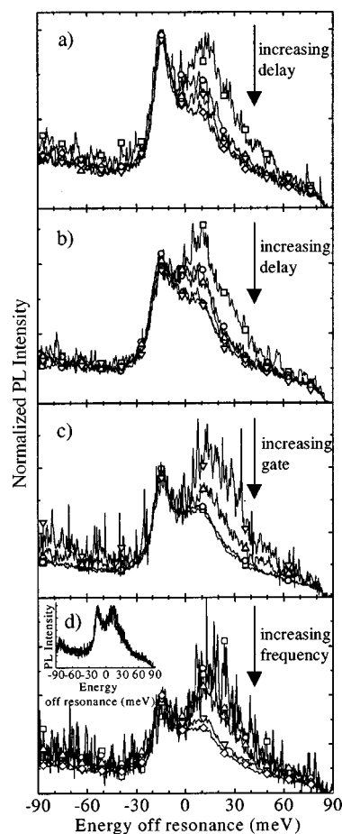
FIG. 5. Gated PL spectra detected after opening of the laser beam normalized to the lower polariton peak. (a) 4.2 K, 10 Hz chop rate, 0.5 ms detection time windows delayed by 0 ms ( \square ), 0.5 ms ( \circ ), 2 ms ( \triangle ), 5 ms ( \nabla ), cw ( \diamond ). (b) 80 K, 10 Hz chop rate, 0.5 ms detection time windows delayed by 0 ms ( \square ), 0.5 ms ( \circ ), 2 ms ( \triangle ), 5 ms ( \nabla ), cw ( \diamond ). (c) 4.2 K, 50 Hz chop rate, 0 ms delay, detection time windows of 500 \mu\text{s} ( \square ), 250 \mu\text{s} ( \circ ), 100 \mu\text{s} ( \triangle ), 50 \mu\text{s} ( \nabla ). (d) 4.2 K, 0 ms delay, 0.5 ms detection time window at chop rates of 2 Hz ( \square ), 5 Hz ( \circ ), 10 Hz ( \triangle ), 20 Hz ( \nabla ), 50 Hz ( \diamond ). The inset shows three normalized spectra measured at different excitation intensities (0.75, 1.125, and 1.5 \text{ kW/cm}^2 ) (0 ms delay, 0.5 ms gate, 10 Hz chop rate).
