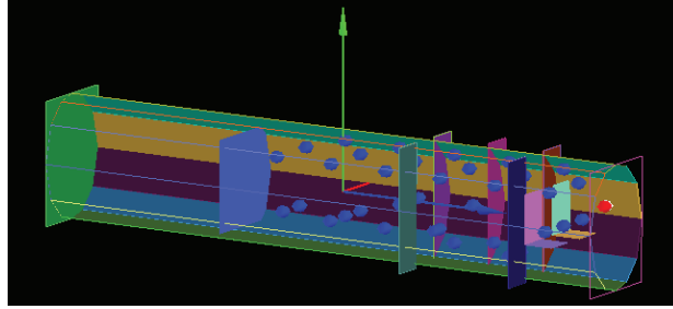
Figure 1: The figure shows the Rockwell T-39 Sabreliner with transmitter placed in the front dash board as shown by the red dot and 34 receivers placed throughout the cabin as shown by blue dots.
