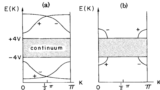
FIG. 2. Bound states of the trion and their dispersion in 2D. Energy is relative to that of an exciton; continuum is that of a free hole. (a) Narrow valence bandwidth |V/C| = \nu < \nu_c'' , with + labeling bonding and - antibonding branches. (b) \nu_c' < \nu < 1 . The momentum K is along the [1,1] direction.
