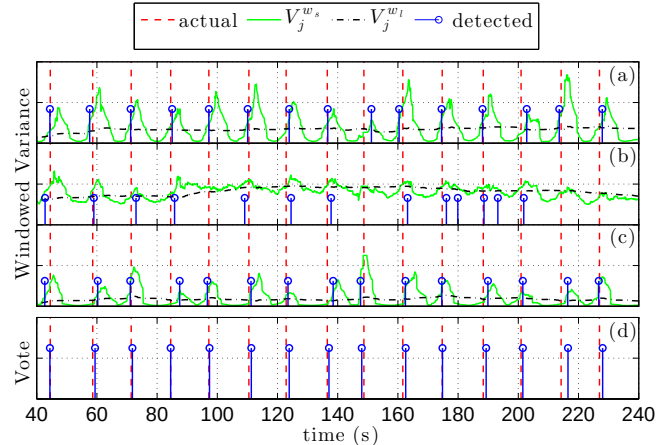
Figure 4: The majority vote over transmitter-receiver antenna pairs reduces false alarms and missed detections. (a), (b), and (c) show the results of the windowed variance based line crossing detection for three antenna pairs using WiFi. In (d), we see that the majority vote eliminates false alarms and missed detections.
