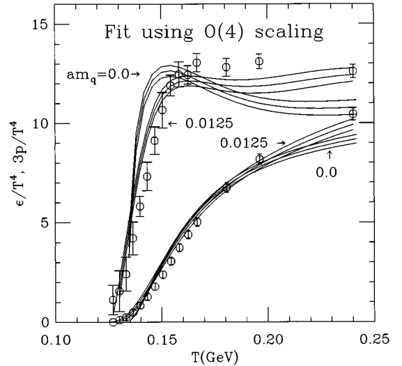
FIG. 10. The am_q=0 equation of state from a fit to the data that includes the O(4) universal scaling function. Also shown are the data and the fit at am_q=0.0125 for comparison. Again, there is only a weak mass dependence. The ‘‘bump’’ just after the transition is likely an artifact of the extrapolation. The solid lines correspond to the central value and a one standard deviation above and below this result (statistical errors only).
