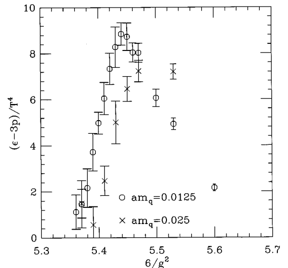
FIG. 7. The interaction measure \varepsilon - 3p .
