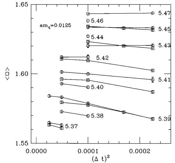
FIG. 2. The plaquette expectation value as a function of the step size squared, \Delta t^2 , and the gauge coupling. Results are shown for am_q=0.0125 . Octagons denote hot lattices ( 6/g^2 is given for each) and squares denote cold lattices.
