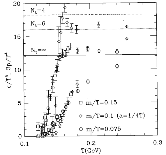
FIG. 9. The equation of state along lines of constant m_q/T . The octagons denote am_q=0.0125 results, squares am_q=0.025 . The diamonds indicate an earlier result on N_t=4 lattices. Horizontal lines correspond to Stefan-Boltzmann laws for N_t=4, 6 , and the continuum. The energy density increases rapidly near the crossover while the pressure (lower curve for each symbol) rises smoothly.
