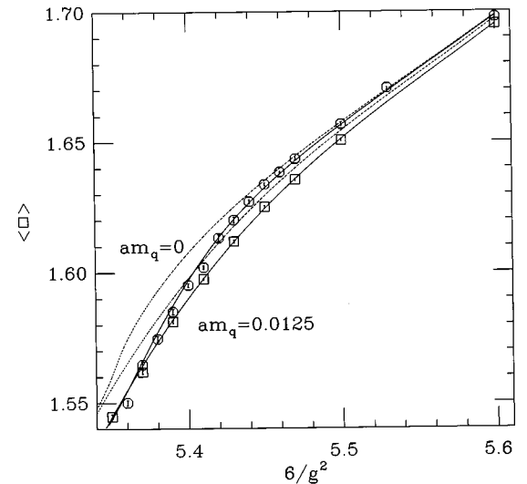
FIG. 3. The plaquette expectation value as a function of the gauge coupling at am_q=0.0125 . Octagons denote hot lattices, squares cold lattices. The area between the curves gives the pressure while the difference at each point is related to the interaction measure. The lines are from a fit including the O(4) singular free energy described in the text (dashed lines are an extrapolation to am_q=0 ).
