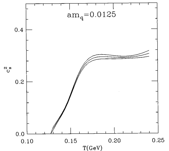
FIG. 11. The speed of sound squared from a fit to the data that includes the O(4) universal scaling function. c_s^2 rises rapidly in the crossover region and then approaches the free gas result 1/3. The low temperature result is probably not accurate (see text). The solid lines correspond to the central value and a one standard deviation above and below this result (statistical errors only).
