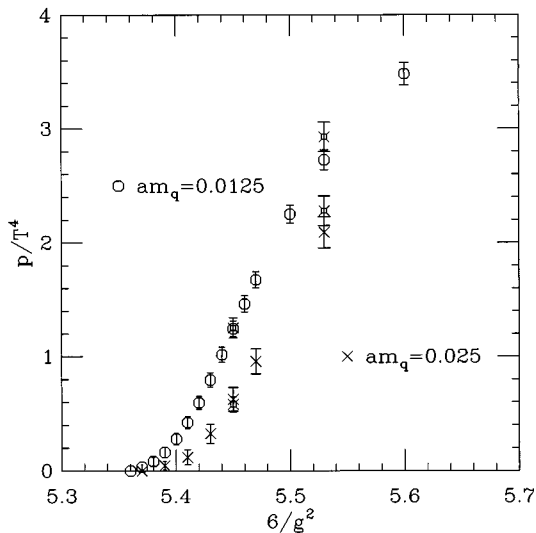
FIG. 6. The pressure obtained from integrating \langle\Box\rangle with respect to 6/g^2 at constant am_q . The values from the quark mass integrations (fancy squares) are also shown for comparison.
