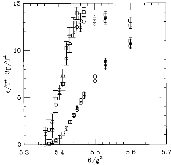
FIG. 8. The energy density constructed from I+3p (upper two curves). Also shown is 3p (lower two curves) and results with no step size extrapolations (squares). The difference is the step size systematic error in the equation of state. The data are for am_q=0.0125 only. The fancy squares denote 3 times the pressure as calculated from the integration of \langle\bar{\psi}\psi\rangle with respect to am_q .
