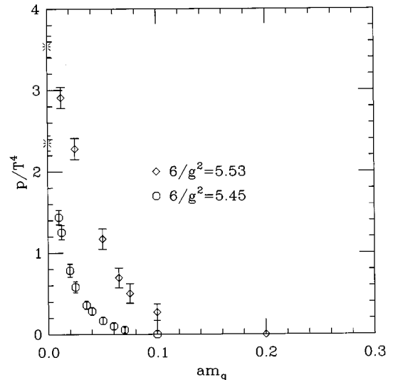
FIG. 5. The pressure obtained from integrating \langle \bar{\psi}\psi \rangle with respect to am_q and constant 6/g^2 . The values at zero quark mass (bursts) are obtained by setting \langle \bar{\psi}\psi \rangle=0 on the hot lattices and extrapolating \langle \bar{\psi}\psi \rangle to am_q=0 on the cold lattices.
