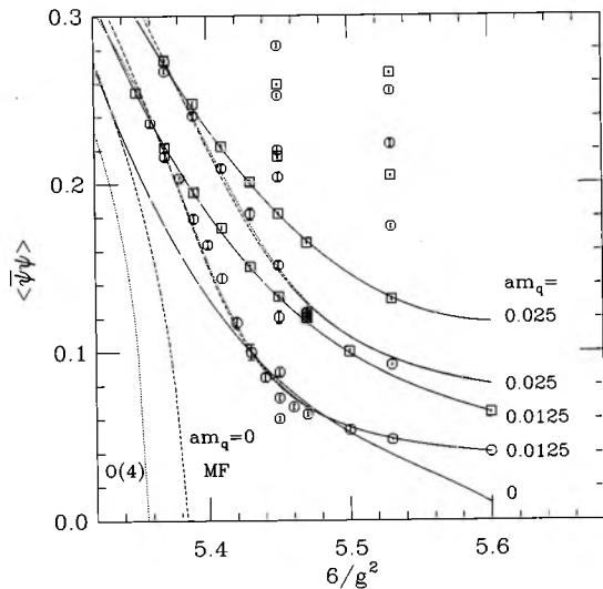
FIG. 4. \langle \bar{\psi}\psi \rangle as a function of 6/g^2 and am_q . The difference in the hot (octagons) and cold (squares) values is related to the interaction measure. \langle \bar{\psi}\psi \rangle on the hot lattices also serves as an order parameter for the system. Lines depict fits to O(4) and mean field singular forms of the free energy plus analytic terms to \langle \square \rangle , \langle \bar{\psi}\psi \rangle , and their derivatives [Eqs. (5)–(8)]. Only points with am_q \leq 0.025 were included in the fits. The difference between O(4) (dotted line) and mean field forms (dashed line) is not discernible at the quark masses where simulations were run. Extrapolations to m_q=0 , however, give different critical couplings. Solid lines correspond to polynomial fits to the cold data and the corresponding extrapolation to am_q=0 .
