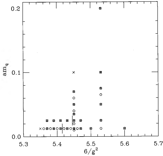
FIG. 1. Phase diagram for our simulations. The vertical solid lines indicate approximate locations of the crossover. Crosses indicate cold lattices, octagons hot lattices.
