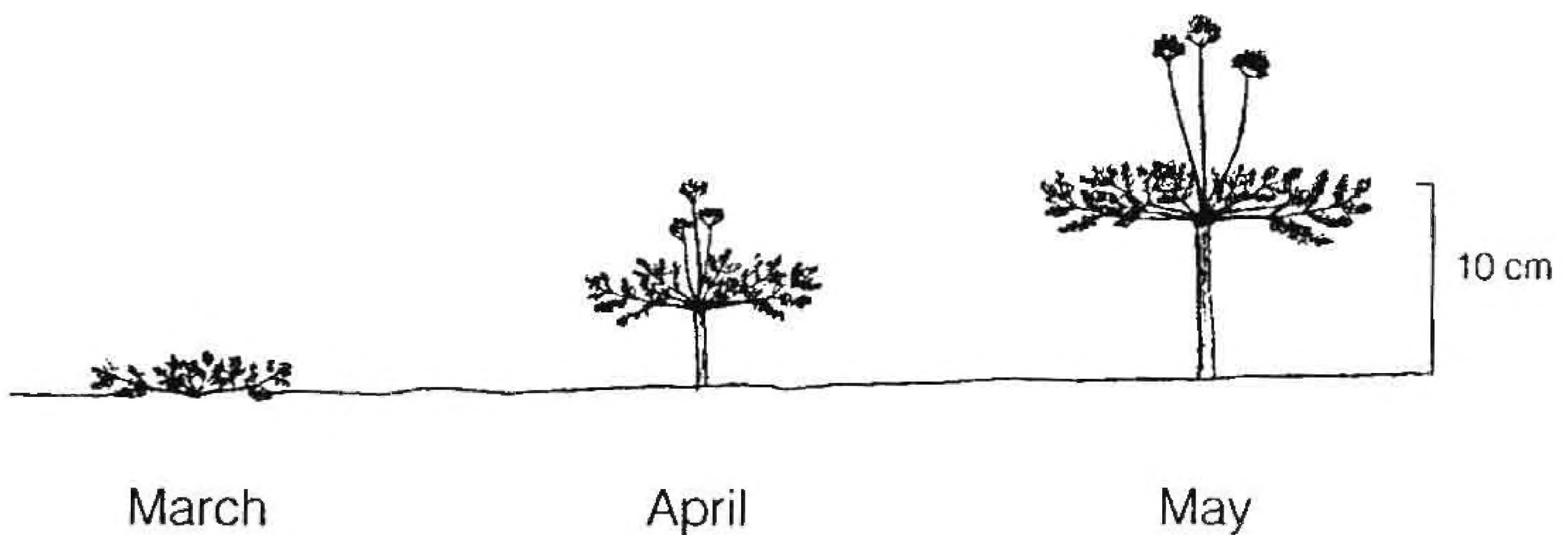
Fig. 13. Height of Cymopterus longipes above the ground surface at different months during the spring growing season. After Werk et al. (1986).
