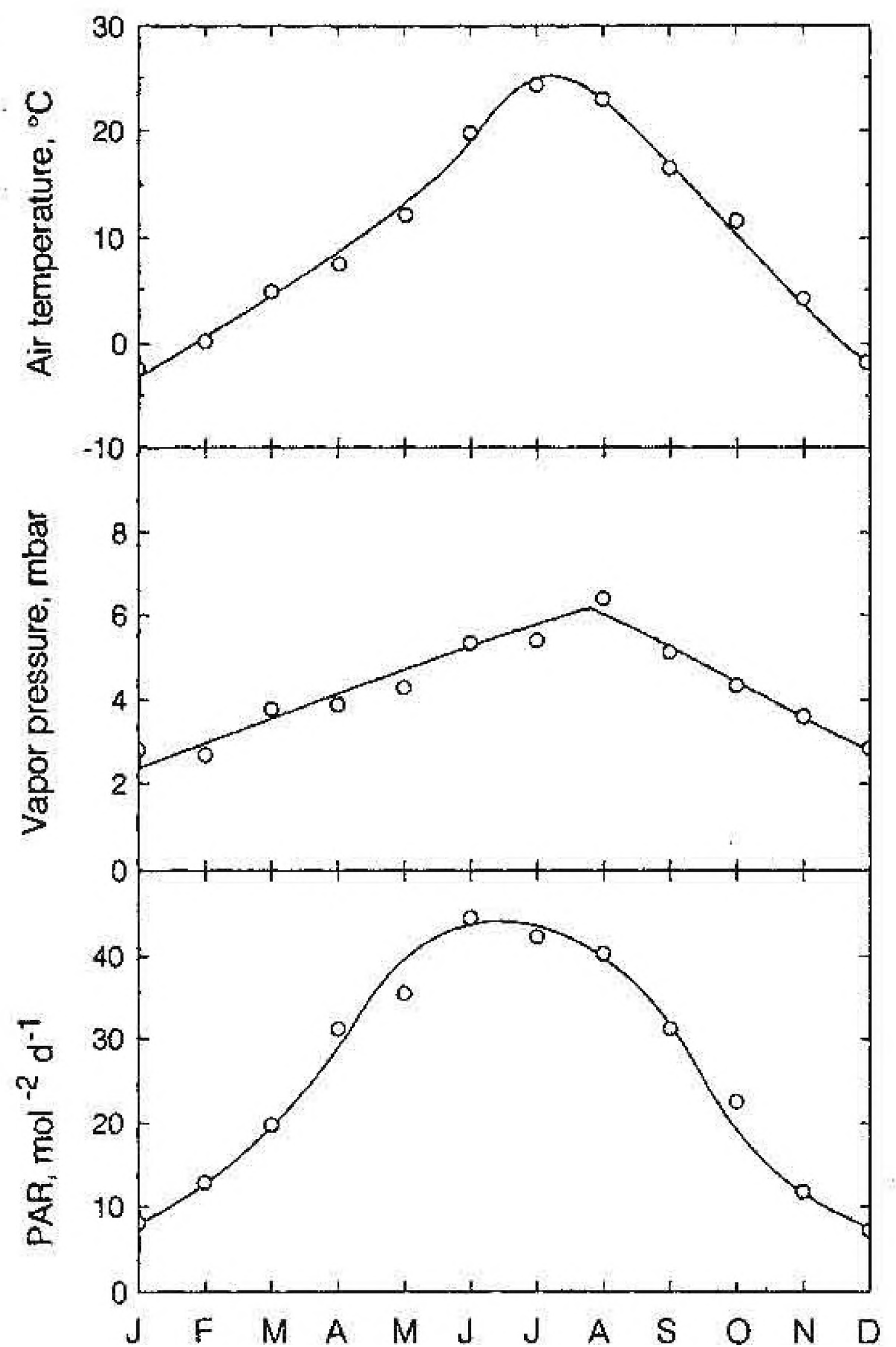
Fig. 8. Mean monthly air temperature, vapor pressure, and photosynthetically active solar radiation (400-700 nm) measured at Red Butte #2 between 1982 and 1990.
