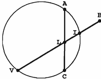
Figure 4.4: Simple geometric relations can be used to rank landmark configurations.
