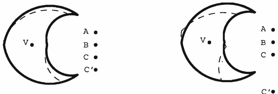
Figure 3.11: Both graphs show an error bound of \pm 30\% in visual angle estimate with the viewpoint 5 units from configuration. The dark lines surround the area of uncertainty for the ABC configuration. The dashed lines surround the area for the ABC' configuration.
