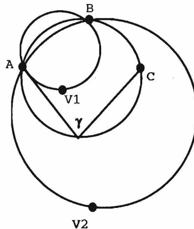
Figure 4.24: Visual angle to A and C is larger than \gamma at V_1 and smaller than \gamma at V_2 .
