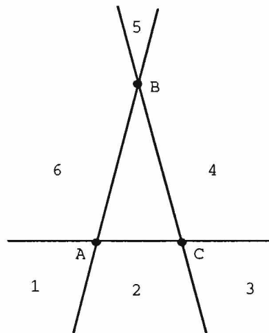
Figure 3.26: A partial ordering of non-linear features limits the orientation regions in which the viewpoint can lie.
