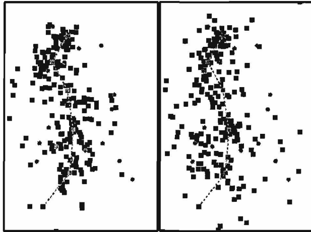
Figure 4.15: Results after 50 trials with error bounds of \pm 30\% in visual angle measure. The heuristic is used for choosing landmarks in the frame on the left.
