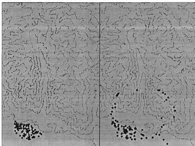
Figure 4.8: Scatter plots of 100 viewpoint estimates for the viewpoint shown in the foreground of Figure 4.7. The plot on the left is the result of localizing using a good landmark configuration. The plot on the right is the result of choosing configurations at random. The map boundaries were 427890E, 4482180N by 452160E, 4498320N UTM coordinates. The maps are shown with east toward the top.
