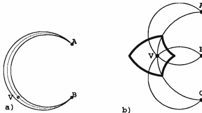
Figure 3.5: The error in visual angle estimate to two points constrains the viewpoint V to a) a thickened ring. When three points are used, the viewpoint is constrained to b) the intersection of two such thickened rings.
