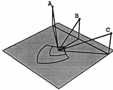
Figure 3.19: Visual angles to A, B, and C of 45^\circ and an error bound of \pm 10^\circ produce the larger area of uncertainty. The smaller area is what would result with the same visual angles and error amounts if the features were in the same plane as the viewpoint.
