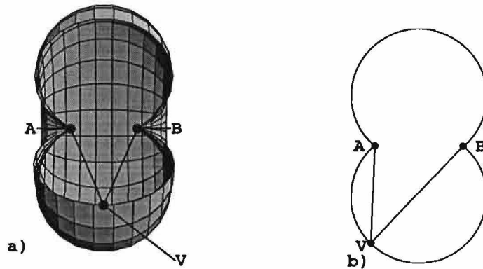
Figure 3.3: Knowledge of the visual angle measure between two points, A and B, constrains the viewpoint V to a) a surface of revolution. If a two-dimensional approximation of the environment is assumed, the viewpoint is constrained to b) the intersection of the surface in a) with a plane through A, B, and V.
