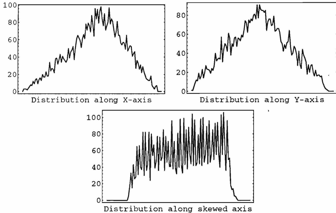
Figure 4.18: Distribution of points along x-axis, y-axis and along an axis rotated 45° counterclockwise from the x-axis.
