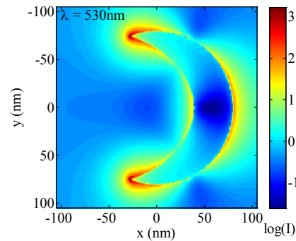
Figure 3 – Near Field Pattern at Dipole Resonance
