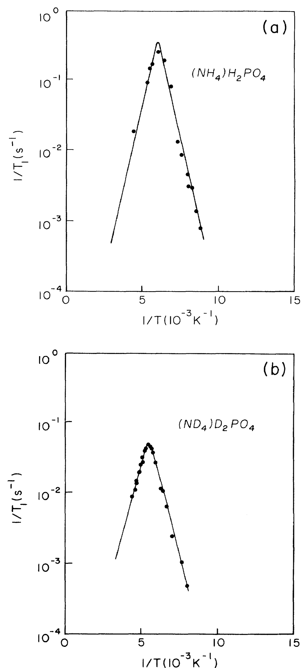
FIG. 1. The spin-lattice relaxation rates as a function of 1/T in (a) pure ADP and (b) pure DADP. Note that only a single peak is observed in each case. This peak corresponds to ammonium motions in these compounds. The solid curves are merely to guide the eye.
