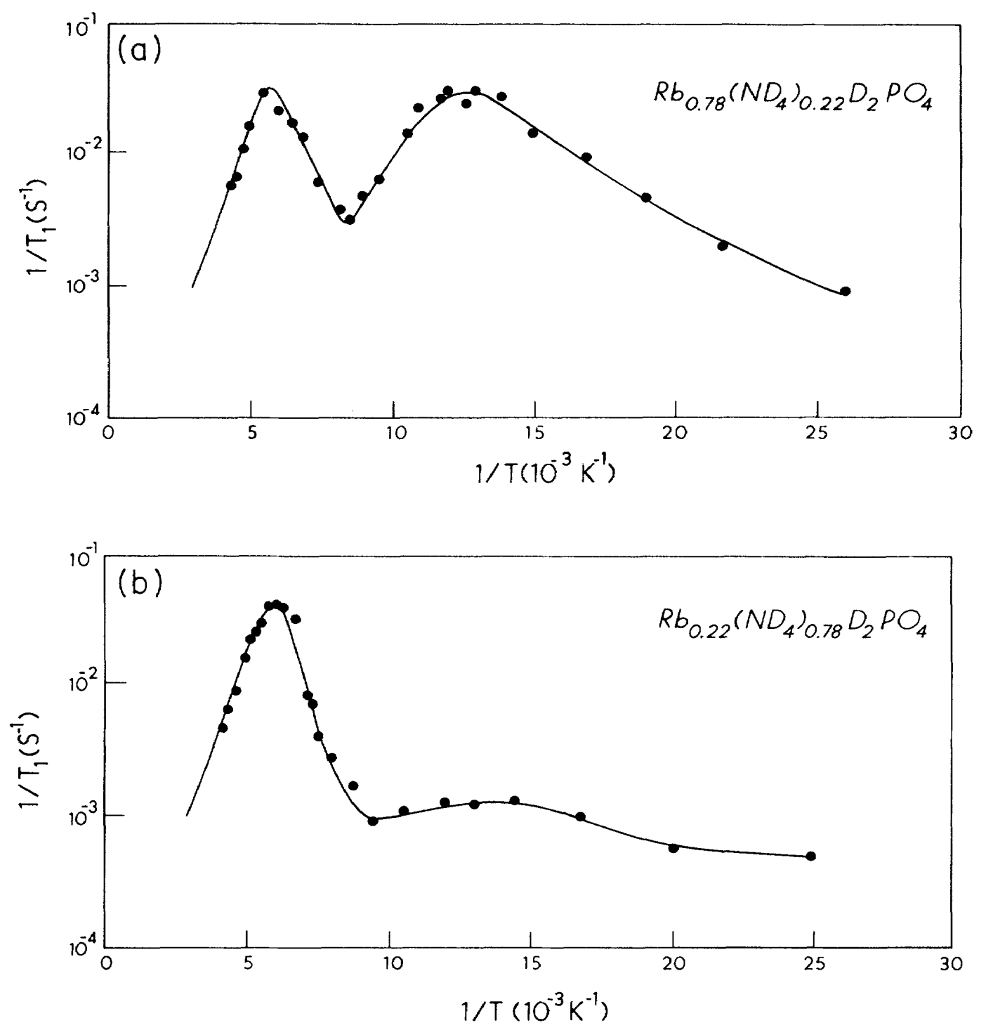
FIG. 3. The spin-lattice relaxation rate as a function of 1/T in DRADP mixed single crystals having (a) x=0.22 and (b) x=0.78 . The solid curves are merely to guide the eye.
