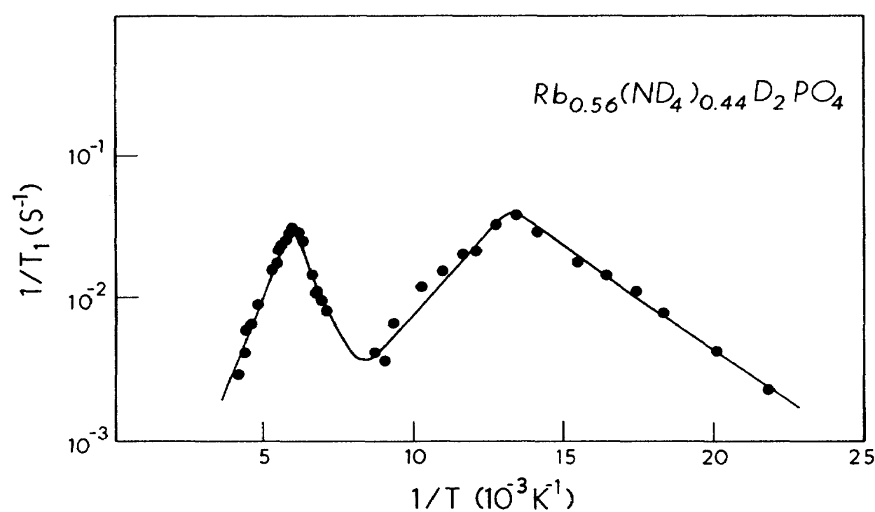
FIG. 2. The spin-lattice relaxation rate as a function of 1/T in the mixed single-crystal DRADP having x=0.44 . Note that two T_1^{-1} maxima were observed in this system. The one at high temperatures is driven by ammonium motions and the one at low temperatures is due to the slowing-down of O—D \cdots O motions. The low-temperature one is absent in pure ADP or RDP. The solid curve is merely to guide the eye.
