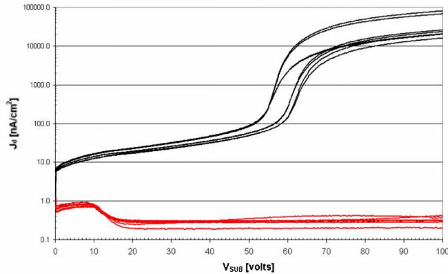
Fig. 7. Current-voltage measurements on 2 \text{ mm}^2 p-i-n diodes fabricated on the same wafers as the CCDs, and also fabricated on wafers with undoped poly backseal gettering. The high dark currents were seen on a standard thickness, 650\text{--}675 \mu\text{m} thick wafer fully finished at DALSA Semiconductor. The low dark current data is for a 250\mu\text{m} thick wafer finished at LBNL with an approximately 20 \text{ nm} thick ISDP layer on the backside of the wafer.
