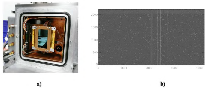
Fig. 8. a) Photograph of a 4\text{k} \times 2\text{k} , 15 \mu\text{m} pixel CCD installed in a test dewar. b) Image taken after a 30 minute exposure under dark conditions. The substrate bias voltage was 100\text{V} and the operating temperature was -140^\circ\text{C} . The CCD thickness is 250 \mu\text{m} and the wafer was finished at LBNL.
