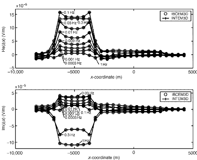
Figure 10. Model 2. Plots of the real and imaginary parts of the sum of electric fields E_x^{\Delta\sigma_p} and E_x^{\Delta\sigma_a} along the x -directed profile at y = 1250 m. The solid lines represent the results obtained by INTEM3D; the circles show the data computed by IBCEM3D.
