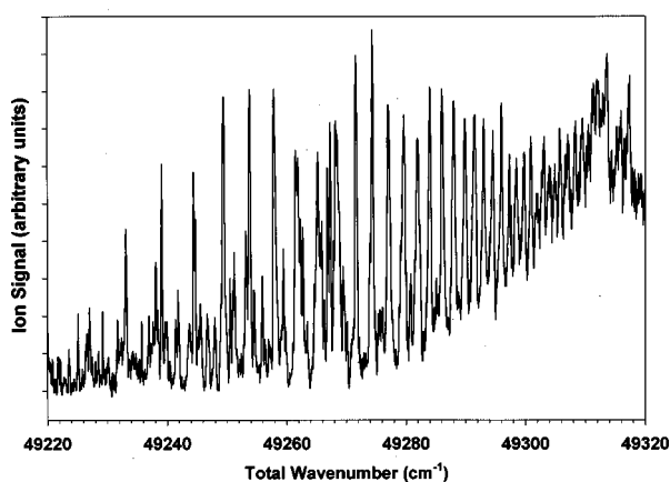
FIG. 2. An example of the Rydberg spectra collected for YO. In this scan, the first tunable laser was set to the R_1(6) excitation of the A^2\Pi_{1/2}, v' = 0 \leftarrow X^2\Sigma^+, v'' = 0 band, thereby populating the J'(A) = 7.5e level of the A^2\Pi_{1/2}, v' = 0 state. The second laser was then scanned near the ionization threshold, and high Rydberg states were exposed by pulsed field ionization and time-of-flight mass spectrometric detection of the resulting YO^+ cations. The strongest lines correspond to Rydberg states converging to J^+ = 8 , while many of the weaker lines correspond to Rydberg states converging to J^+ = 6 . Although other weak lines are present, they cannot be readily identified as Rydberg states converging to a particular rotational level of the cation.
