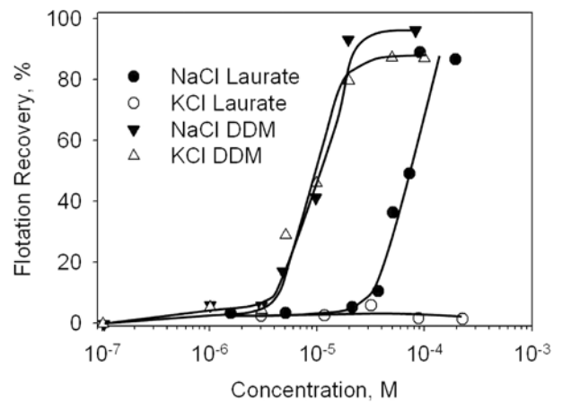
Figure 13 — Flotation of KCl and NaCl in their saturated brine as a function of sodium laurate and DDM (sodecyl amorpholine) concentration (Miller et al., 1992; Hancer et al., 2001).
