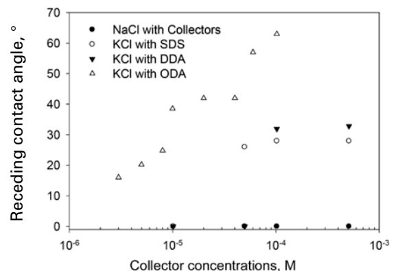
Figure 7 — Captive bubble contact angles of saturated brines at KCl and NaCl salt surfaces with the addition of different collectors (Cao et al., 2010).
