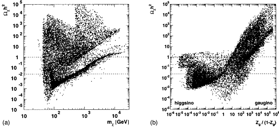
FIG. 3. Neutralino relic density including neutralino and chargino coannihilations versus (a) neutralino mass m_\chi and (b) neutralino composition Z_g/(1-Z_g) . The horizontal lines bound the cosmologically interesting region 0.025 < \Omega_\chi h^2 < 1 .
