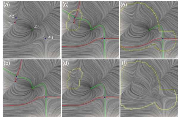
Figure 6: SyntheticA. (a) The original vector field: sinks are red, sources are green and saddles are blue. (b) The topological skeleton: saddle-sink separatrices are red and saddle-source separatrices are green. (c)-(d) 1st level simplification: before (c) and after (d) Smoothing . (e)-(f) 2nd level simplification: before (e) and after (f) Smoothing .
