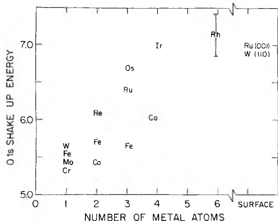
FIG. 5. Plot of the energy separation between the O-1s peak and the most intense shake-up peak in the photoelectron spectra of TM carbonyls (condensed), as a function of the number of metal atoms in the carbonyl. The data points are indicated by the chemical letters identifying the metal atoms (Table I).
