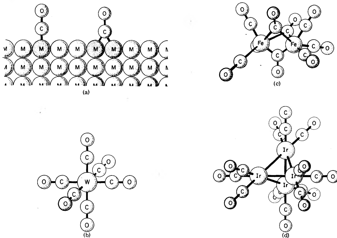
FIG. 1. Ball and stick structures of CO bound to a transition metal: (a) a solid surface with terminal and bridge-bonded CO, (b) W(CO)_6 , (c) Fe_2(CO)_9 with three bridge-bonded CO molecules, and (d) Ir_4(CO)_{12} .
