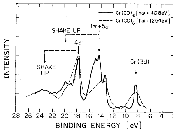
FIG. 7. Comparison of the gas phase Cr(CO) 6 valence-band spectrum taken at \hbar\omega = 40.8 eV with the spectrum obtained using \hbar\omega = 1254 eV.
