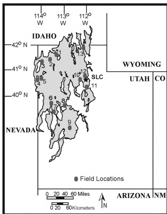
Figure 1. Lake Bonneville at highstand 15,000 ^{14}\text{C} yr ago and tufa locations examined in this study. 1 = north end of the Hogup Mountains, 2 = Terracc Mountain, 3 = Lucin Hill and Lion Mountain, 4 = Wendover Knob, 5 = Volcano Peak and Silver Island tombolo, 6 = north end of Fish Springs Range, 7 = Sand Pass, 8 = Table Mountain, 9 = Black Rock Volcano, 10 = north end of the Oquirrh Mountains, 11 = Point of the Mountain, 12 = Beck Street/Wasatch fault, 13 = Cutler Dam; SLC = Salt Lake City.
