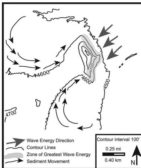
Figure 3. Schematic example of wave energy orienting landforms at Lucin Hill. In this case, a tombolo is formed in the lee of an island, which blocks wave energy and allows a tombolo to form. The windward side of the island shows erosional characteristics as it absorbs the brunt of wave energy.
