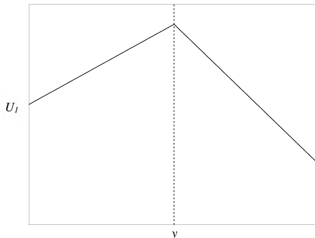
Figure 1. Graphical illustration of the Fehr-Schmidt model. The horizontal axis shows variation in y , the payoff of player 2. The vertical axis shows player 1's utility, U_1 . The payoff of player 1, x , is held constant at the value indicated by the dashed vertical line. To the left of the dashed line, player 1 faces advantageous inequality, the relevant utility function is U_1(x, y) = x - \beta(x - y) , and thus the slope is \beta in this region. To the right of the dashed line, inequality is disadvantageous for player 1, U_1(x, y) = x - \alpha(y - x) , and the slope is -\alpha . This example assumes 0 < \beta < \alpha , and consequently utility reaches its maximum when y = x .
