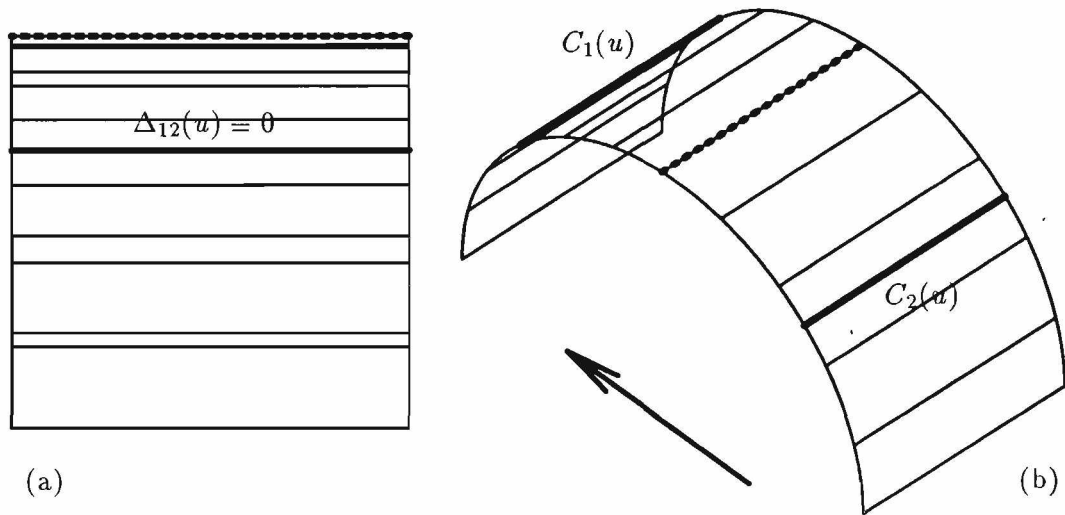
Figure 3: If S has silhouettes (dotted) in image plane, and only x and y are consulted in \Delta_{12}(u) computation, \Delta_{12}(u) may be found by Algorithm 1 to be wrongly zero, terminating prematurely.
