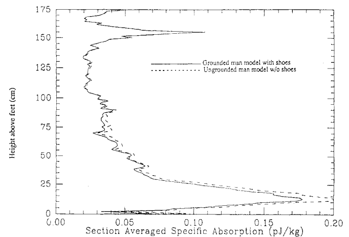
Fig. 10. Variation of section or layer-averaged specific absorption for the ultrawideband pulse of Fig. 2. E_{peak} = 1.1 V/m.
