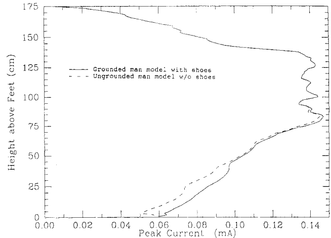
Fig. 9. Peak currents induced in the various sections of the body for grounded shoe-wearing and ungrounded barefoot (isolated) conditions of the model. Incident field is the EMP of Fig. 8. Currents are calculated using (8).
