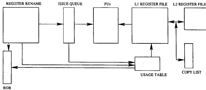
Figure 1. The Two-Level Register File Organization.
