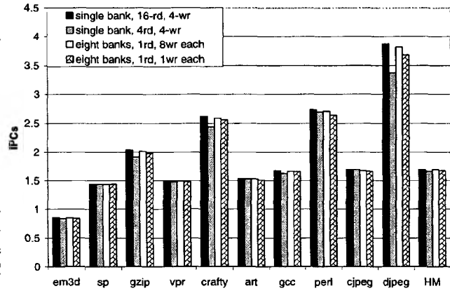
Figure 6. IPCs with eight bank organizations.
