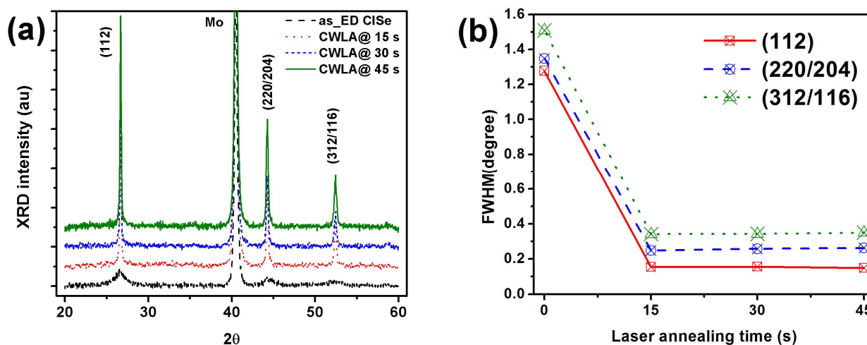
Figure 4. (a) XRD \theta - 2\theta scan of as-ED CuInSe 2 film and CWLA samples for varying annealing time and (b) Change in FWHM values of XRD peaks for varying annealing time.
