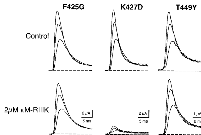
FIG. 3. Mutations in the pore do affect the binding of \kappa\text{M} -conotoxin R11IK to Shaker channels. Upper panel, whole cell currents from oocytes expressing the mutated channel of Shaker H4. Mutating the phenylalanine to glycine (F425G) results in a channel that is insensitive to 2 \mu\text{M} \kappa\text{M} -conotoxin R11IK (left panel). Mutating the lysine 427 to an aspartate (K427D) results in a channel with increased sensitivity to this toxin (middle panel). Mutating the threonine at position 449 to tyrosine (T449Y) results in a channel that is insensitive to 2 \mu\text{M} \kappa\text{M} -conotoxin R11IK. Voltage steps are as described in the legend to Fig. 2.
