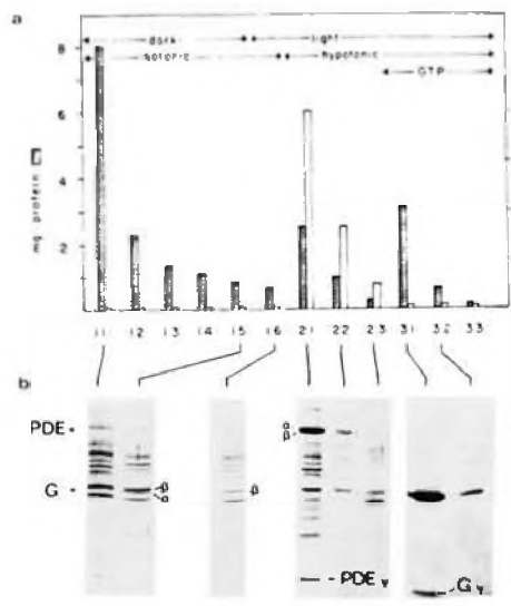
Fig. 1. (a) Elution of ROS-associated proteins with isotonic buffer (1.1-1.6), hypotonic buffer (2.1-2.3), and hypotonic buffer + 40 μM GTP (3.1-3.3). Matched columns: total protein eluted from membrane fragments of 100 retinas. Protein assayed by Coomassie G250 with bovine serum albumin as reference (22). Light columns: PDE activity. (b) Analysis of the supernatants by SDS-PAGE.
