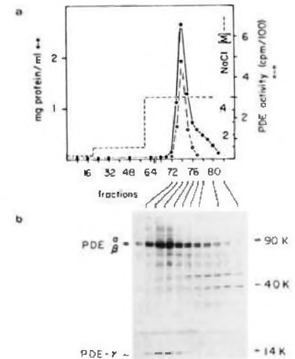
Fig. 2. (a) Chromatography of combined hypotonic supernatants on a DE52/6100 column. Protein is assayed as in Fig. 1. (b) Peak fraction analyzed by SDS-PAGE.
