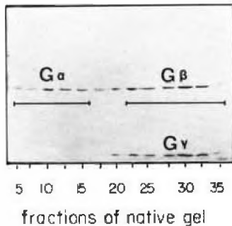
Fig. 4. SDS-PAGE analysis of fractions containing G \alpha and G \beta separated by native gel electrophoresis. The bars mark the fractions pooled.
