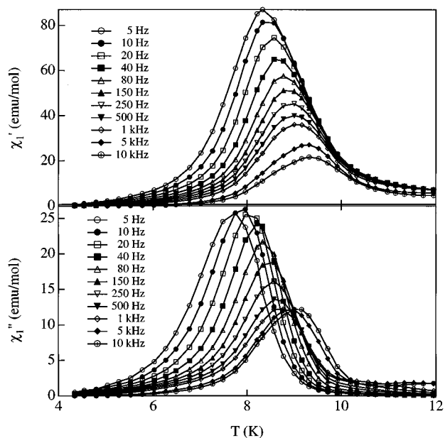
FIG. 2. Real and imaginary parts of \chi_{ac} of 2 for H_{ac}=1 Oe ( H_{dc}=0 ) and 5 \leq f \leq 10\,000 Hz.
