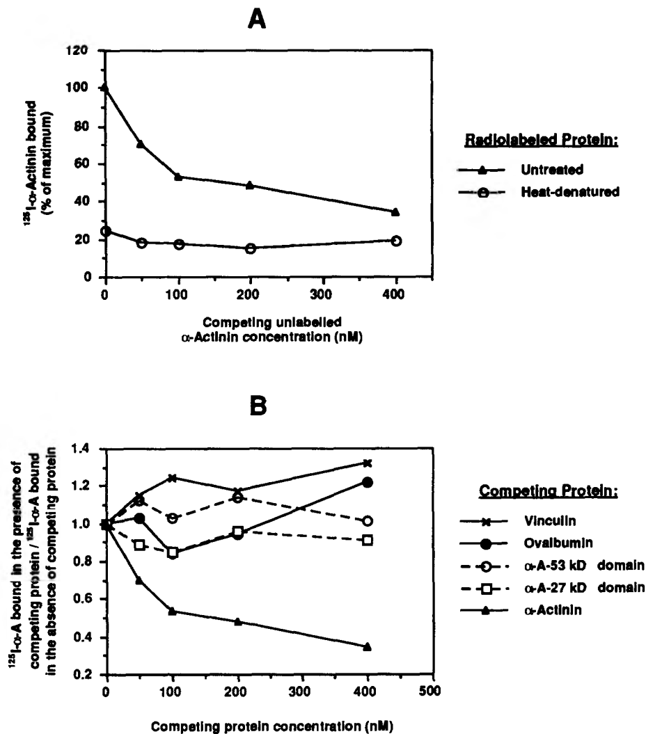
Figure 7. Specificity of the association between zyxin and \alpha -actinin. (A) Comparison of the binding of untreated ( \blacktriangle ) and heat-denatured [ ^{125} I]- \alpha -actinin ( \circ ) to zyxin immobilized on microtiter wells. The data are expressed as a percentage of the maximal binding obtained. (B) Binding of [ ^{125} I]- \alpha -actinin to immobilized zyxin in the presence of increasing amounts of competing protein. Only intact \alpha -actinin effectively competes with radioiodinated \alpha -actinin for zyxin binding. The data are expressed as a ratio of the specific counts bound at each concentration of competing protein to the specific counts bound in the absence of competing protein. Each point represents the average value obtained from duplicate wells in multiple experiments. \alpha -Actinin: n = 4 ; ovalbumin: n = 3 ; 55-kD domain: n = 4 ; 27-kD domain: n = 5 ; vinculin: n = 4 . \alpha -A, \alpha -actinin.
