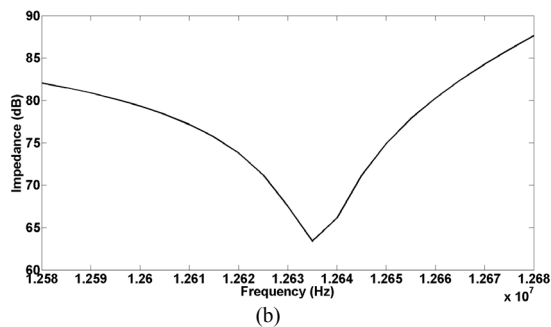
Fig. 7: COMSOL simulation results L = 160 \mu\text{m} , (a) there is a large strain along the length of the device at the frequency of resonance, (b) impedance response of the resonator which resembles impedance response of a series R-L-C circuit.
