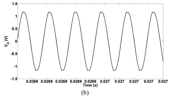
Fig. 9 (a) the input and output voltages of the converter. The high voltage boosting is possible due to the high step up ratio (80) of the PZT [14], (b) voltage waveform at the output of PZT. The switching frequency (56.1 kHz) was slightly higher than the frequency of resonance of PZT (56 kHz). The impedance of the device is the lowest in the neighborhood of resonant frequency. Therefore only the fundamental frequency component can pass through the resonator as evident in Fig. 9b.
