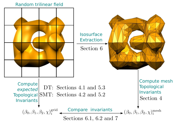
Fig. 1. Overview of our topology verification pipeline. First step, we generate a random trilinear field and extract a random isosurface using the implementation under verification. We then compute the expected topological invariants from the trilinear field and compare them against the invariants obtained from the mesh. We provide two simple ways to compute topological invariants from a trilinear field based on digital topology (DT) or stratified Morse theory.
