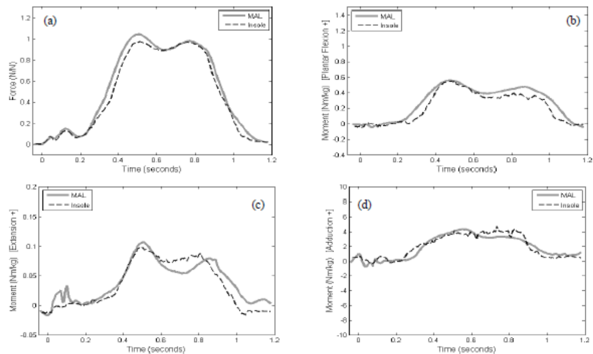
Fig. 3. A representative plot from a stroke subject showing motion analysis lab (MAL) and trained insole results for a) ground reaction force, b) ankle d/p moment, c) knee ev/fl moment and d) knee abd/add moment.
