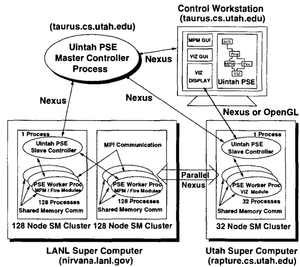
Figure 5: Uintah Architecture Example
