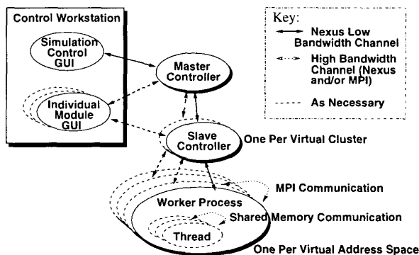
Figure 4: Uintah Parallelization Strategy
