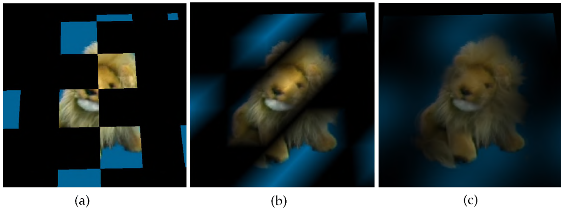
Figure 10: Images of a different basis functions: (a) constant, (b) piecewise linear, and (c) bi-cubic.
