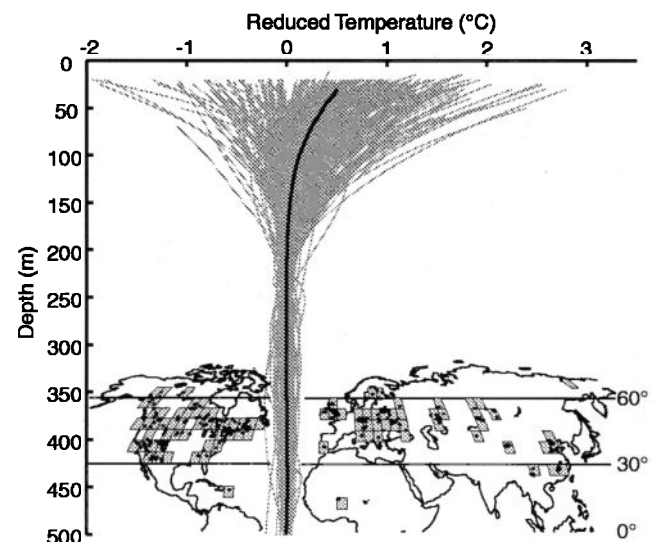
Figure 2. Northern Hemisphere reduced temperature profiles for 1995. Lines represent 439 profiles whose locations are shown in the inset. Bold line shows average reduced temperature profile. The mean SAT record is based on data from the shaded 5 \times 5^\circ grid cells.
