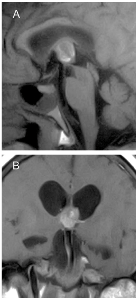
Fig. 1. MR imaging demonstrating mildly enhancing third ventricular mass and non-communicating hydrocephalus. The mass appears to abut the basilar apex on the sagittal and coronal images. A: Sagittal T1-weighted pre-gadolinium MR image; B: coronal T1-weighted post-gadolinium images.
