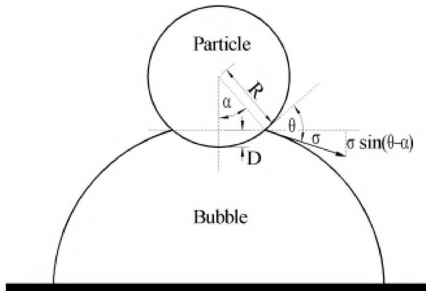
Fig. 4. The equilibrium state of a spherical particle at the air-water interface. ( R ) – particle radius, ( D ) – distance of penetration into air bubble, ( \sigma ) – surface tension, ( \alpha ) – central angle, and ( \theta ) – contact angle
