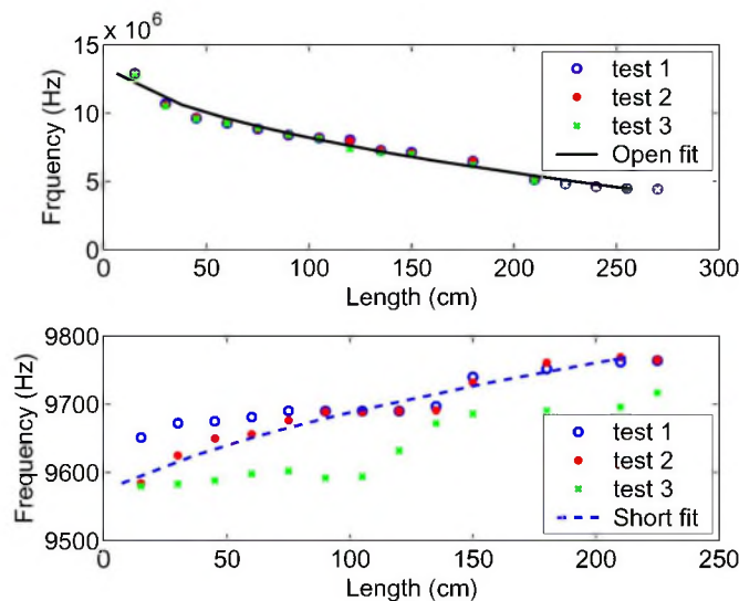
Fig. 8. Length versus output frequency for open- and short-circuited wires using the Schmitt trigger circuit.
