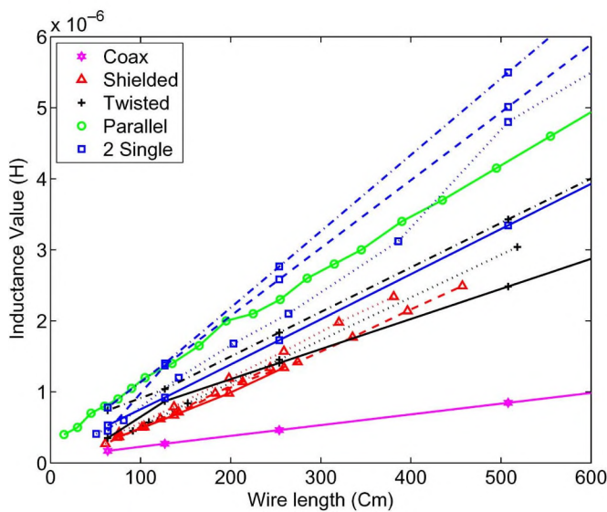
Fig. 2. Measured inductance versus wire length of 13 different open-circuited aircraft wires given in Table I.
