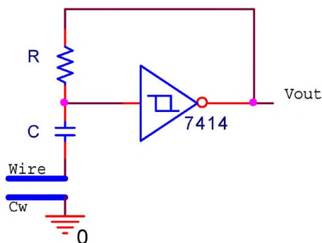
Fig. 7. Schmitt trigger oscillator with capacitor C for short-circuited-wire measurements and without capacitor C for open-circuited-wire measurements.
