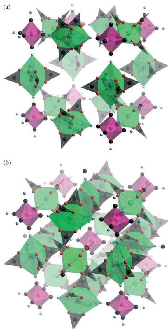
Fig. 1 Single, noninterpenetrating [\text{Ru}_2(\text{O}_2\text{CMe})_4]_3[\text{Cr}(\text{CN})_6] cubic lattice (a), and the observed interpenetrating [\text{Ru}_2(\text{O}_2\text{CMe})_4]_3[\text{Cr}(\text{CN})_6] cubic lattices (b).
