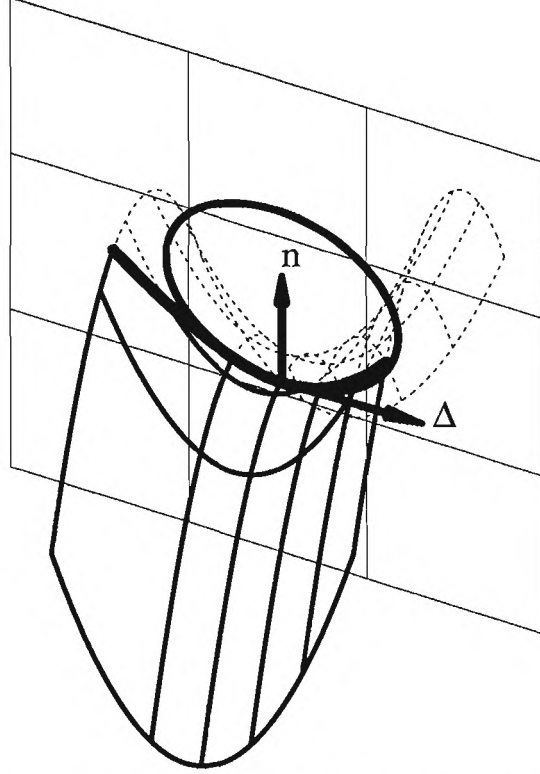
Figure 2: Normal curvature \kappa_n (circle) of F(u, v) at (u, v) in direction \Delta .
