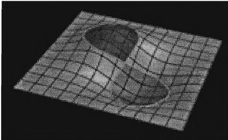
Figure 5: Bicubic surface trichotomy: same control mesh as Figure 3.
