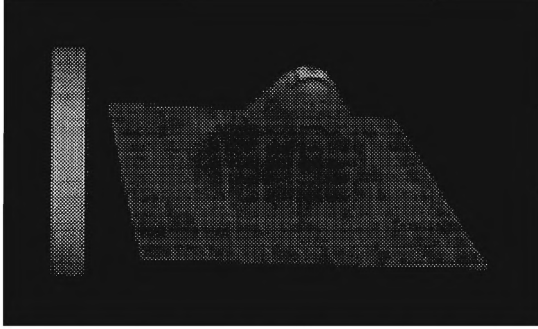
Figure 11: Curvature estimate using surface dichotomy, for the surface in Figure 9.
