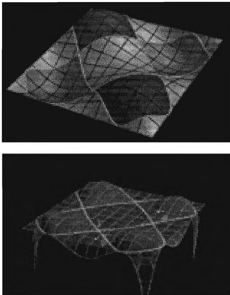
Figure 7: Bicubic surface with convex and concave regions meet at a single point (top). The surface second fundamental form property surface and its zero set (bottom).
