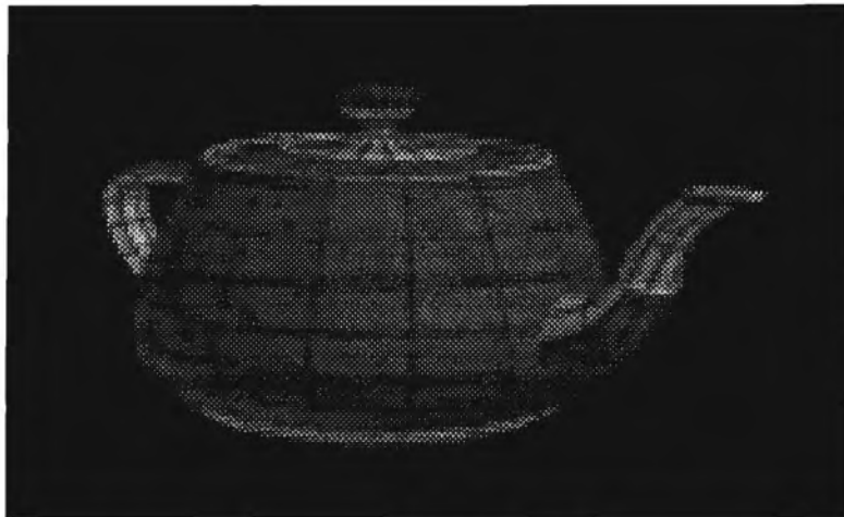
Figure 8: Teapot trichotomy is degenerated into a ditochomy - no concave regions exist.
