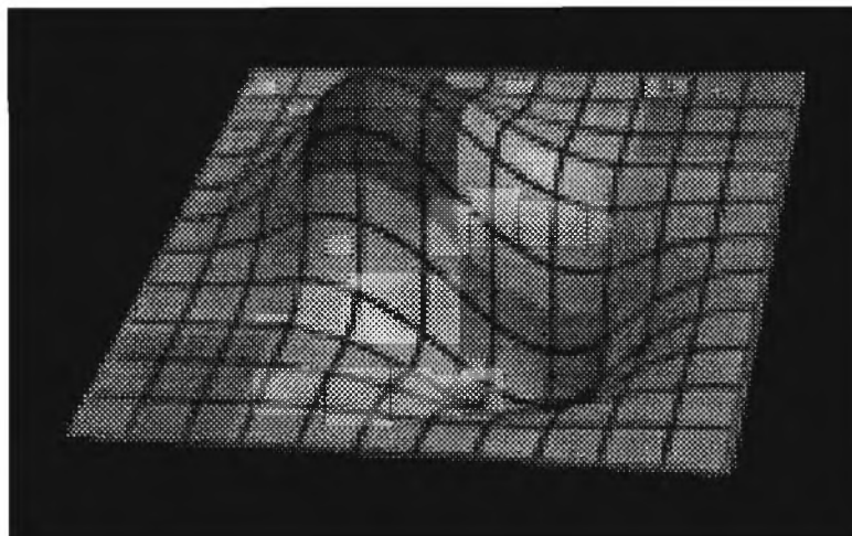
Figure 3: Biquadratic surface trichotomy with 16 polynomial patches.
