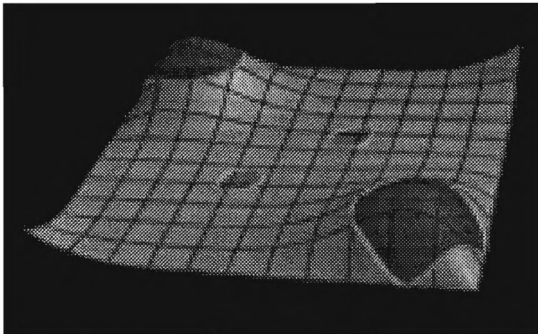
Figure 6: Bicubic with isolated convex and concave regions surrounded by saddle region.
