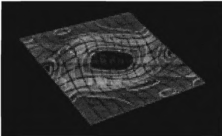
Figure 13: The surface is subdivided into regions with different curvature bounds.
