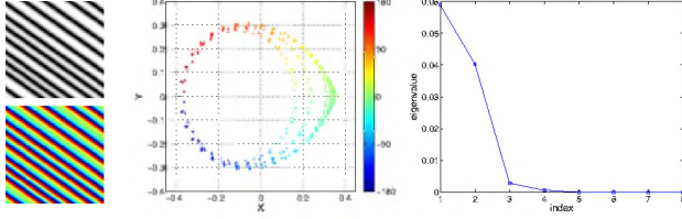
Fig. 1: Projection of the manifold of 5 \times 5 image neighborhoods. Left: Image from which the patches were obtained (top), and phase image of the projected points (bottom). Middle: Patches projected onto 2-D color coded by phase. The colors match those in the phase image. Right: First 8 PCA eigenvalues versus the number of embedding dimensions.
