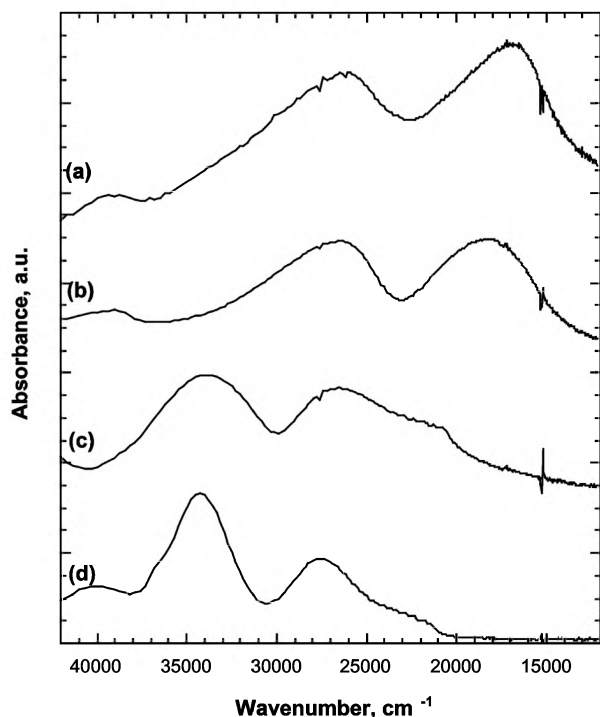
Fig. 4 UV spectra for [\text{Et}_4\text{N}]_2[\text{TCNE}]_2^2 (a), [\text{Pr}_4\text{N}]_2[\text{TCNE}]_2 (b), and [\text{Pr}_4\text{N}]_2[\text{TCNE}][\text{I}_3] as a KBr pellet (c), and in MeCN (d).
