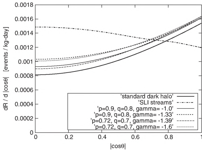
FIG. 12. The folded directional recoil rate dR/d|\cos\theta| off a \text{CS}_2 target for the standard dark halo (thick solid line), SLI streams (thick dash-dotted line), and four logarithmic-ellipsoidal anisotropic models in which the Solar System is on the major axis of the density ellipsoid (solid, thick dotted, dashed, and dotted lines, with parameters given in the legend). In all cases, the reference direction is opposite to the direction of the galactic rotation, (\lambda_{\text{axis}}, \beta_{\text{axis}}) = (167^\circ 340, -59^\circ 574) .
