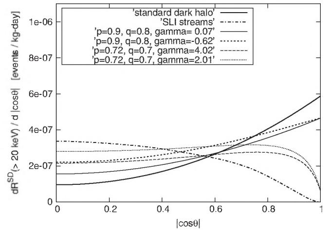
FIG. 14. The spin-dependent folded directional recoil rate dR^{SD}/d|\cos\theta| off a \text{CF}_4 target using a detector with threshold energy equal to 20 keV, for the standard dark halo (thick solid line), SLI streams (thick dash-dotted line), and four logarithmic-ellipsoidal anisotropic models in which the Solar System is on the minor axis of the density ellipsoid (solid, thick dotted, dashed, and dotted lines, with parameters given in the legend). In all cases, the reference direction is opposite to the direction of the galactic rotation, (\lambda_{\text{axis}}, \beta_{\text{axis}}) = (167^\circ 340, -59^\circ 574) .
