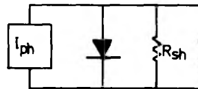
FIG. 3. Schematic diagram of the equivalent circuit for the solar-cell model of the open-circuit voltage induced in a n - i junction by illumination.
